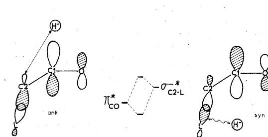
Figure 8. — Secondary interactions for anti- and syn-periplanar attacks.
